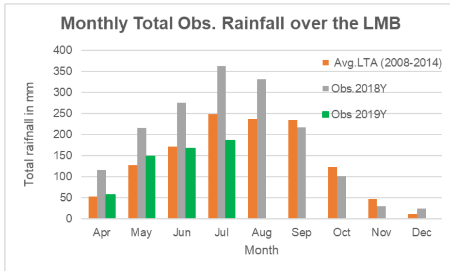
Figure 4: Monthly distributed Rainfall over the LMB
