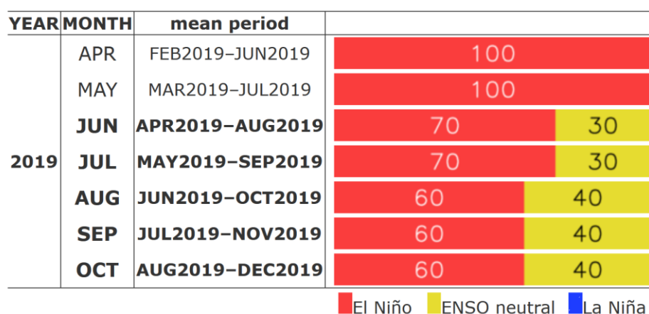
Figure 5 Five-month running mean of the SST deviation for NINO.3 predicted by JMA's El Niño prediction model (JMA/MRI-CGCM2)
